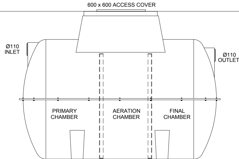
600 x 600 ACCESS COVER
