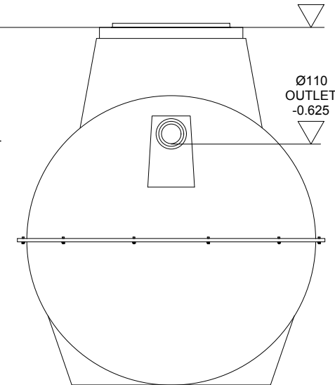
VIEW ON OUTLET
