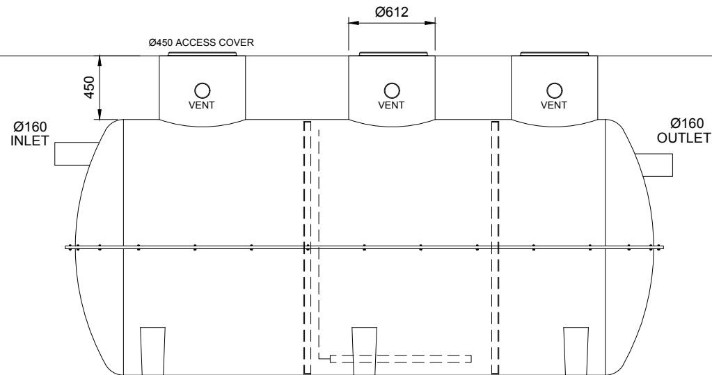
SIDE ELEVATION
