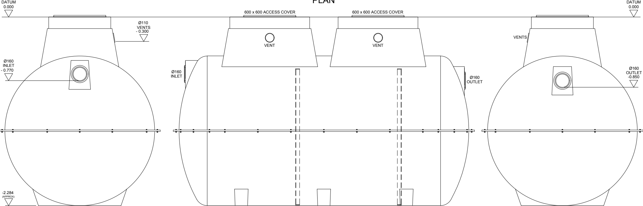
VIEW ON INLET
